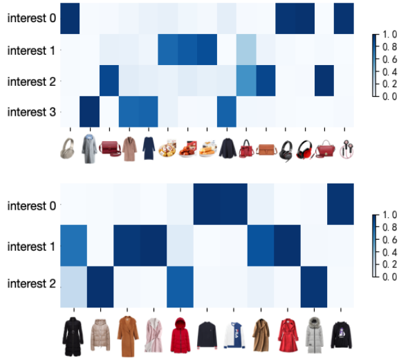
Figure 5: Heatmap of coupling coefficients for two users. Each class of behaviors has the max coupling coefficients on the corresponding interest. User C (upper) and user D (lower) have different granularity of interests.
