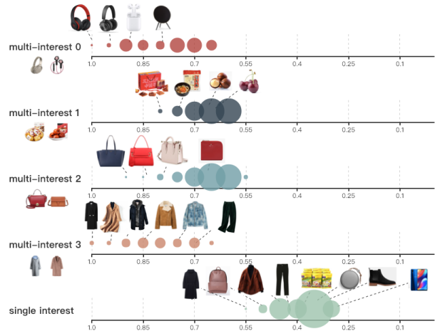
Figure 6: The distribution of items recalled by each interest corresponding to the user behaviors exemplified on the left. Each interest is demonstrated by one axis, of which the coordinate is the similarity between items and interests. The size of the point is proportional to the number of the items with the specific similarity.
