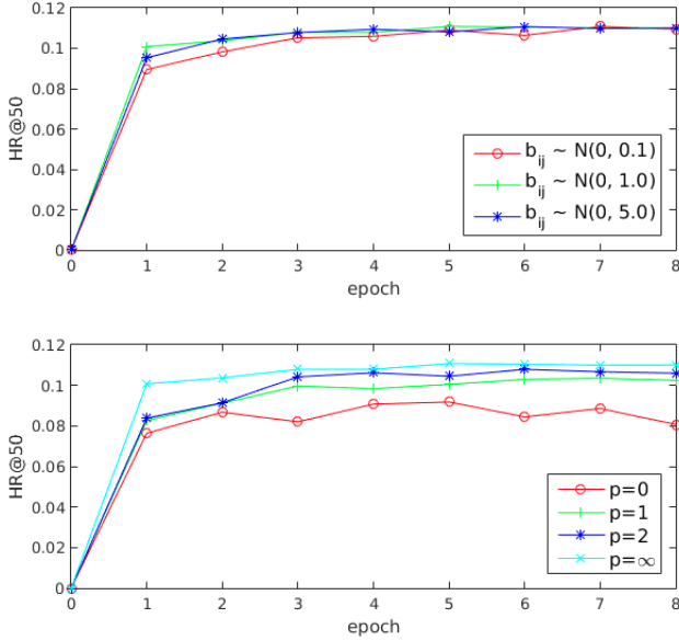
Figure 3: Hyperparameters' impact. The upper part shows that MIND can achieve comparable results with different b_{ij} ; the lower part shows that MIND performs better with bigger p .
